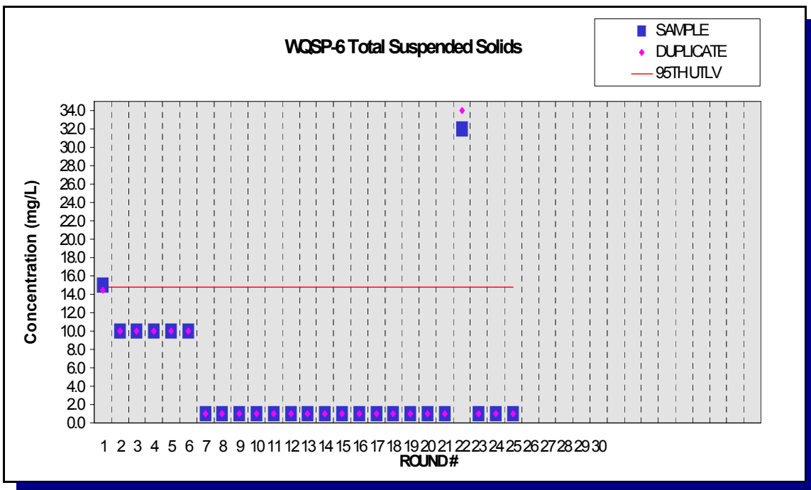
Figure E.84 - Time Trend Plot for Total Suspended Solids at WQSP-6
